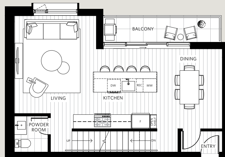
LEVEL 4
