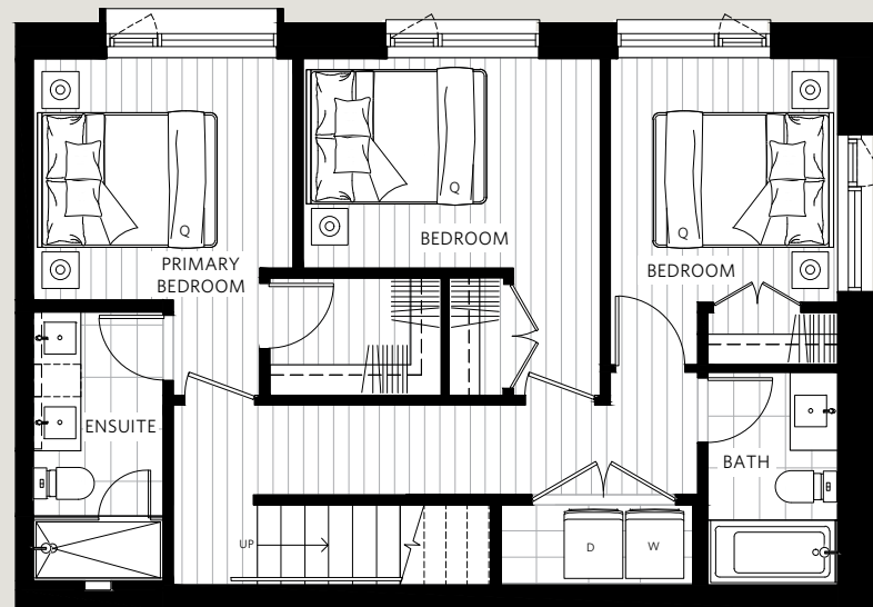
LEVEL 3
